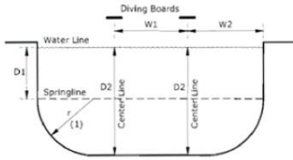
Transverse Section Deep End
